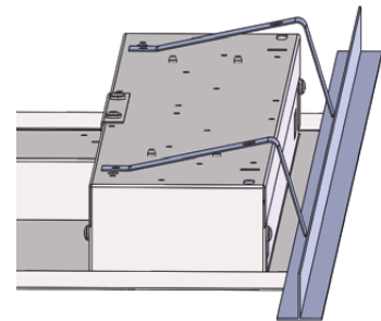
Mounting kit for concealed grid ceiling
